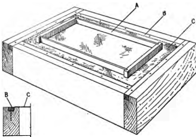
FIG. 2. Drying frame. A sheet of wire gauze of 1 mm. mesh stretched on a heavy wooden frame, being fastened securely in place by a tightly fitting strip of wood which carries the margin of the netting down into a groove in the frame, as shown in the smaller detail drawing. A, molding form of brass bars; B, margin of wire netting and clip fastening it in place; C, wire netting as it clears frame. The wire netting and brass bars are coated with fine shellac.
